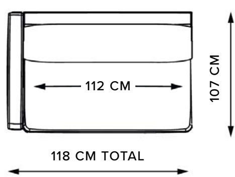
ARMREST SECTION LEFT
